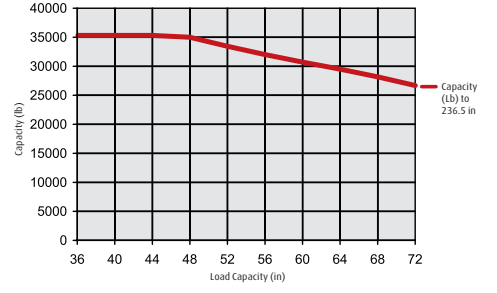
H160-1200 (1401) Load Center Lifting Capacity Diagram
