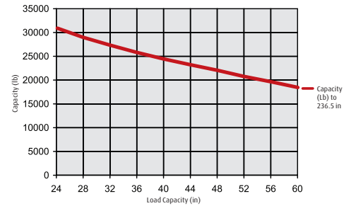
H140 (1401) Load Center Lifting Capacity Diagram
