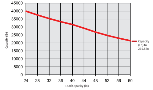
H180 (1401) Load Center Lifting Capacity Diagram
